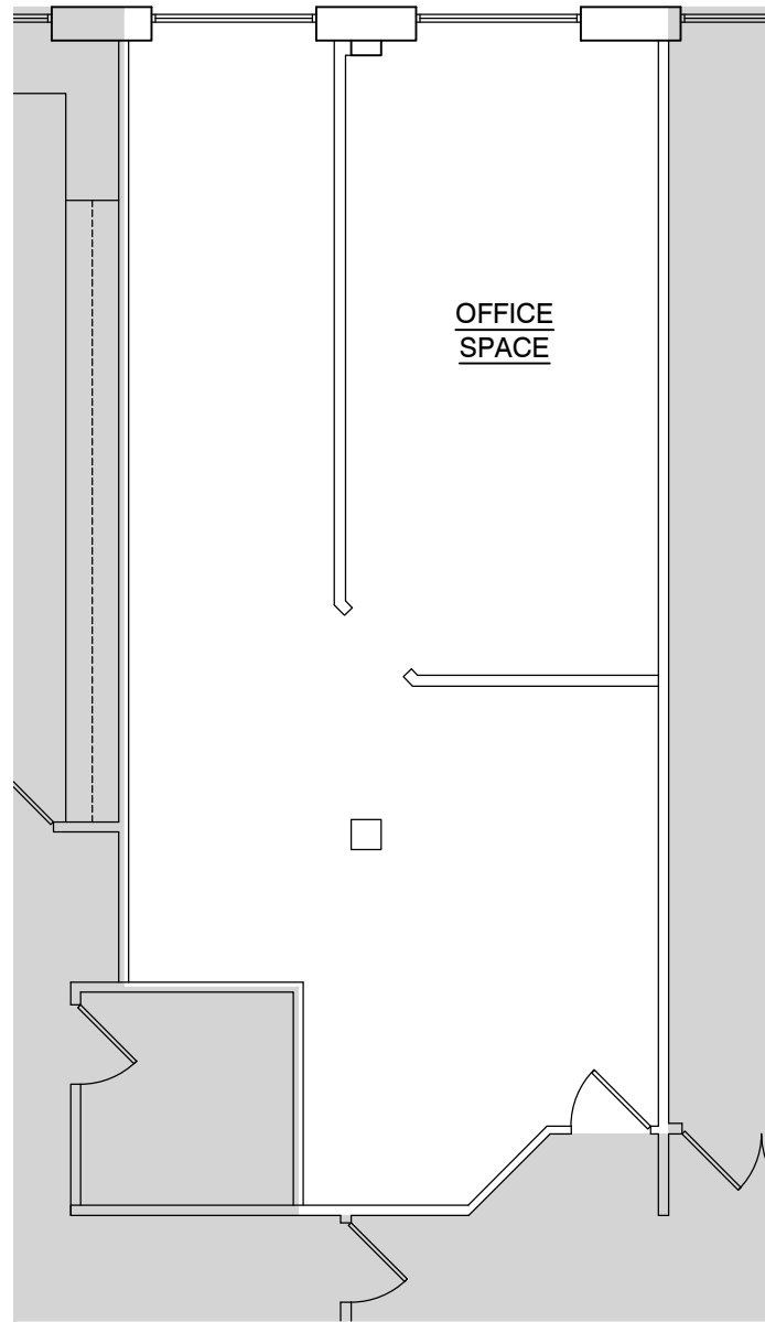
SUITE 320 1/8" = 1'-0"
