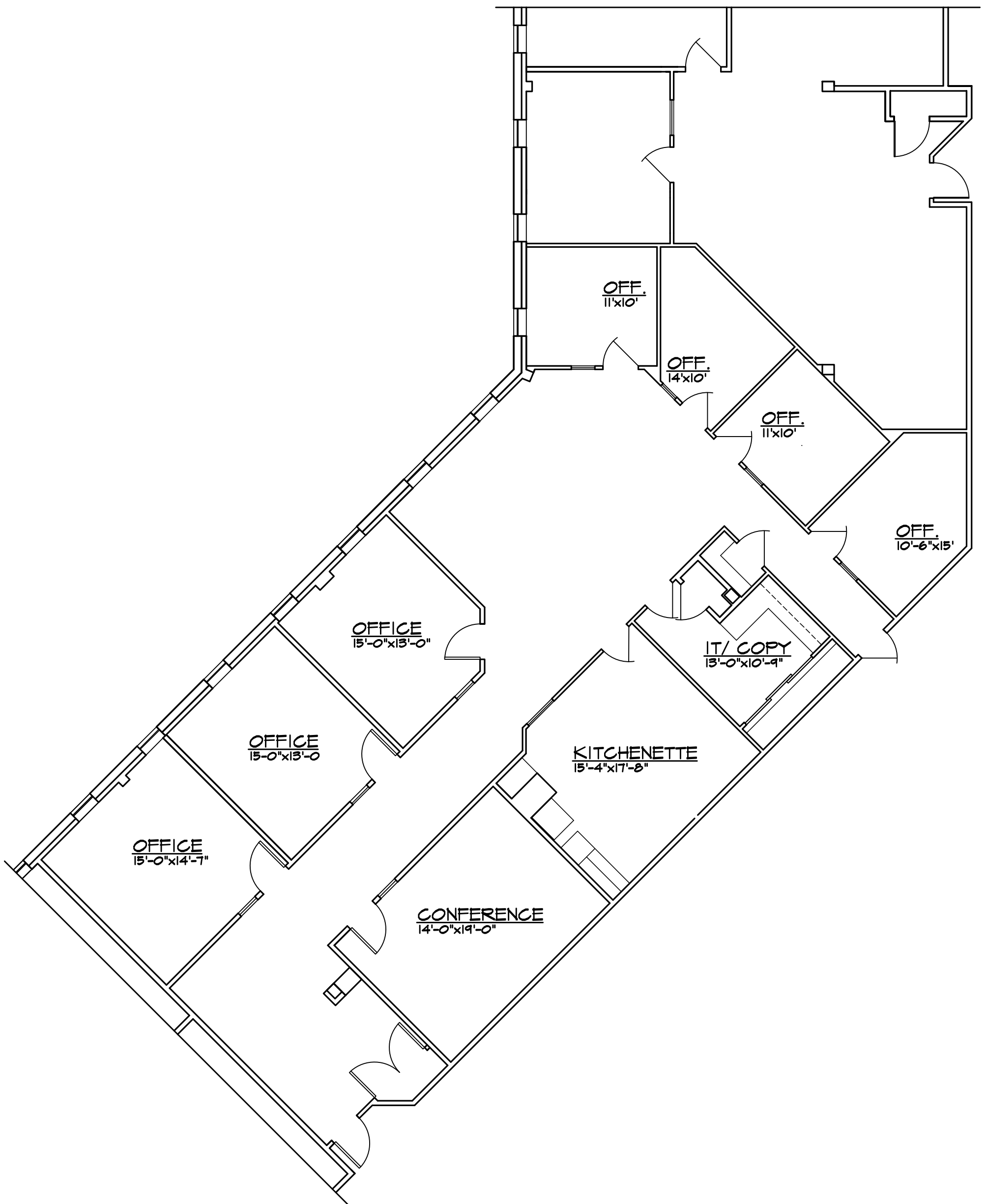
SECOND FLOOR PLAN SUITE 226 SCALE: 1/8" = 1'-0"
