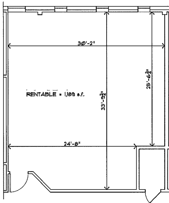
1719 - FIRST FLOOR PLAN SUITE 101 SCALE: 1/8" = 1'-0"
