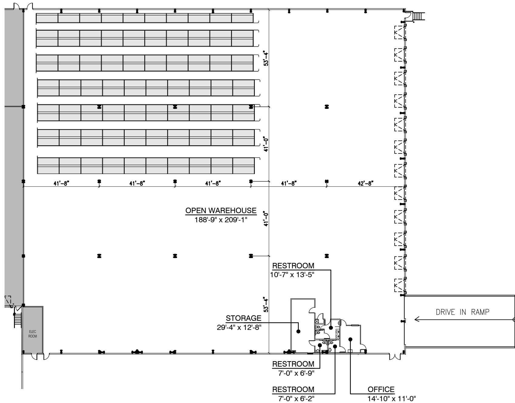
FLOOR PLAN
