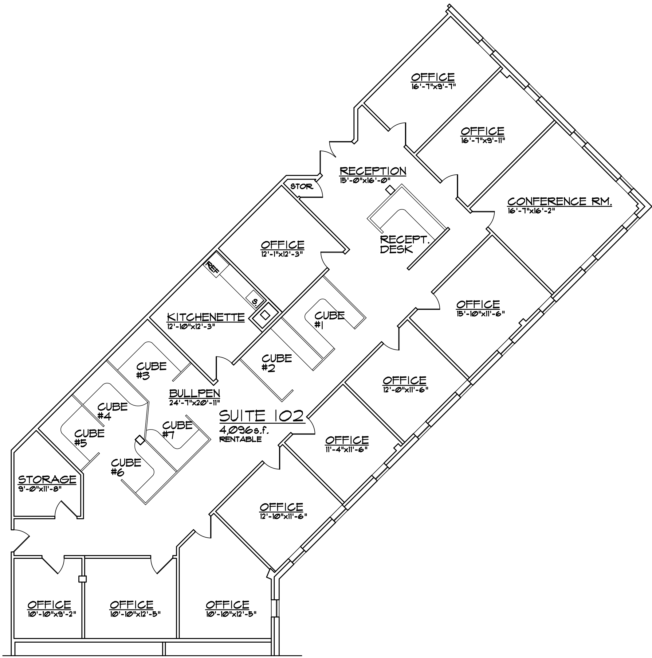
PARTIAL FIRST FLOOR PLAN SUITE 102 SCALE: 1/8" = 1'-0"
